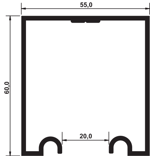
U - 1048 1,453 Kg/m
