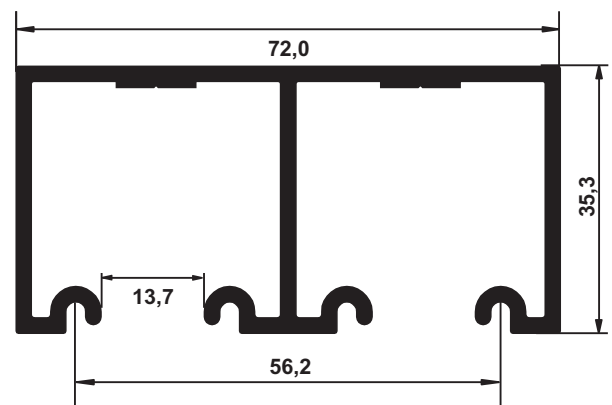
SP - 164 1,294 Kg/m
